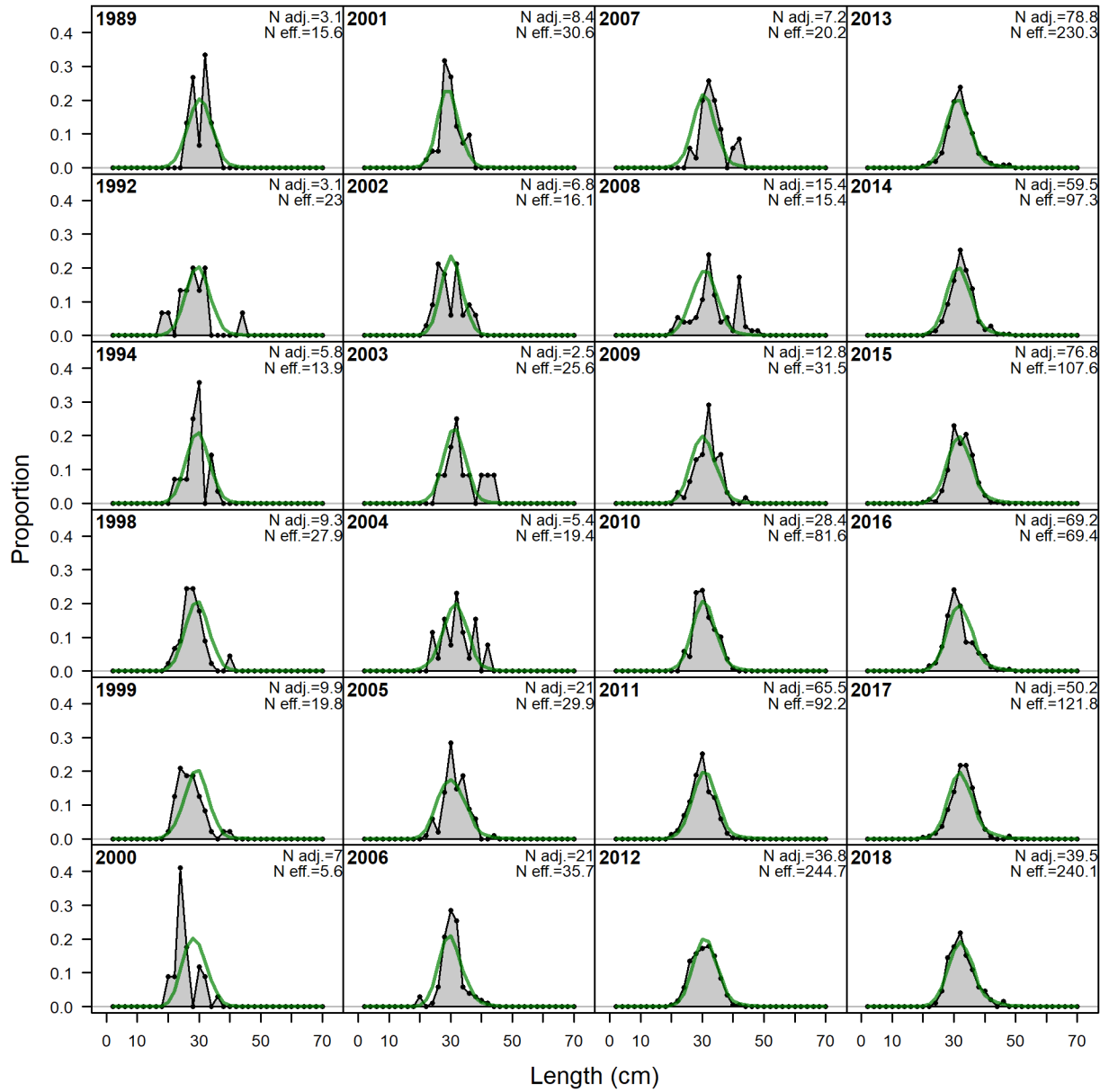
Figure 26. Observed and predicted length compositions (all fish) for Queen Triggerfish in the Commercial Dive fishery. Green lines represent predicted length compositions, while gray shaded regions represent observed length compositions. Input sample sizes (N adj) and effective sample sizes (N eff) estimated by SS are also reported.
