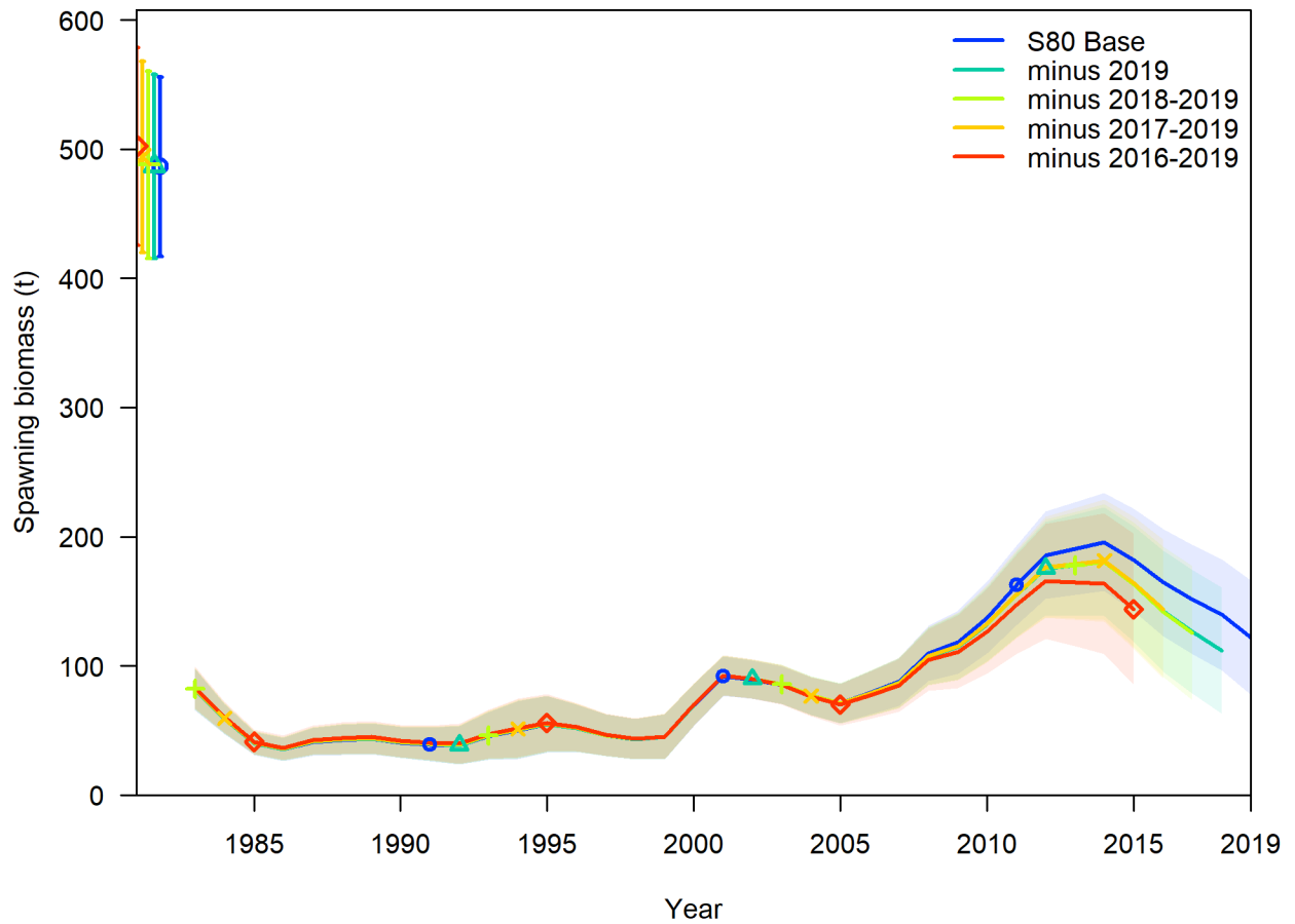
Figure 38. Results of a four-year retrospective analysis for spawning biomass (metric tons) for the Puerto Rico Queen Triggerfish Base Model. There is no discernible systematic bias because each data peel is not consistently over or underestimating any of the population quantities. Shaded area represents the 95% confidence intervals about the model estimate.
