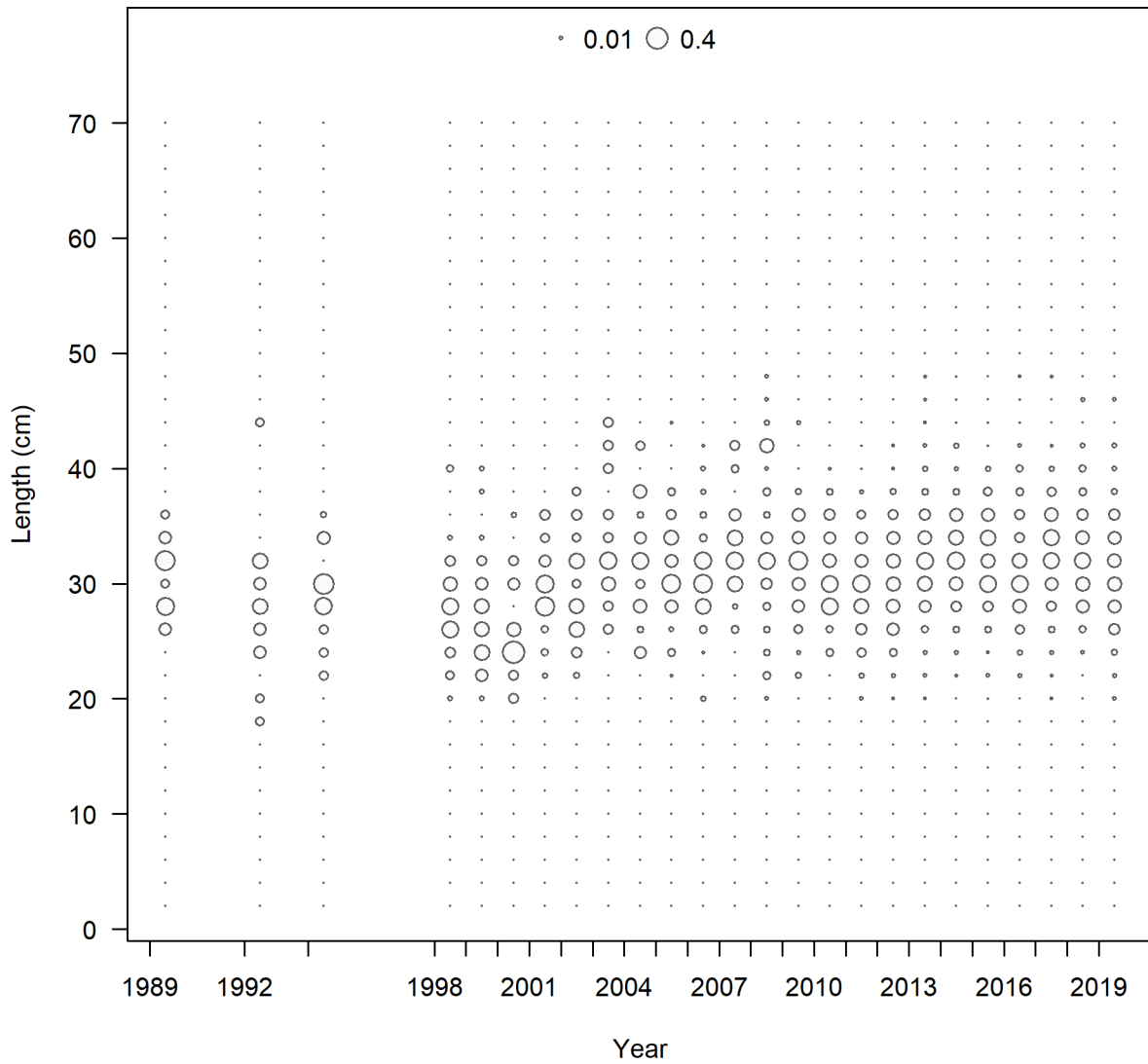
Figure 8. Observed commercial length composition data (all fish) in the Commercial Dive fishery used in the Puerto Rico Queen Triggerfish SS assessment model. Bubble size represents the proportion of length composition data by strata (year).
