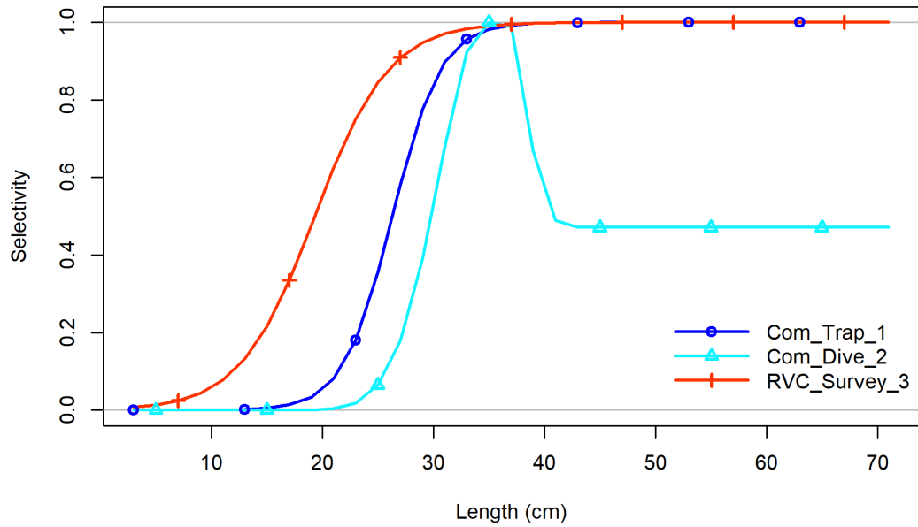
Figure 13. Length-based selectivity for each fleet and survey for Puerto Rico Queen Triggerfish in the terminal year of the assessment (2019).
