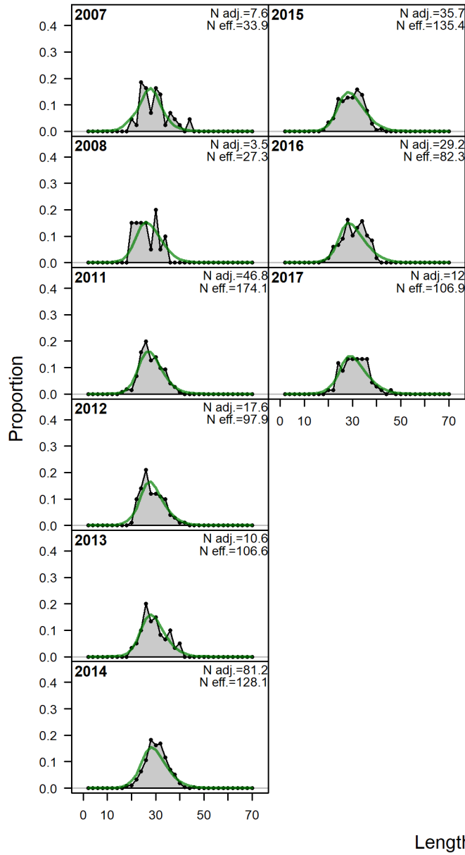
Figure 25 Continued. Observed and predicted length compositions (all fish) for Queen Triggerfish in the Commercial Trap fishery. Green lines represent predicted length compositions, while gray shaded regions represent observed length compositions. Input sample sizes (N adj) and effective sample sizes (Neff) estimated by SS are also reported.
