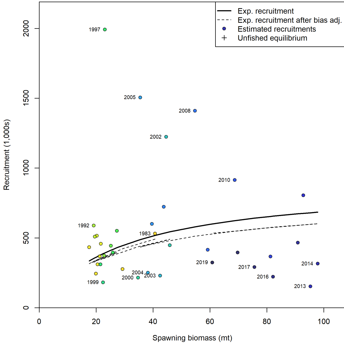
Figure 15. Predicted stock-recruitment relationship (steepness and SigmaR were fixed at 0.7 and 0.6, respectively). Plotted are predicted annual recruitments from Stock Synthesis (circles), expected recruitment from the stock-recruit relationship (black line), and bias adjusted recruitment from the stock-recruit relationship (dotted line).
