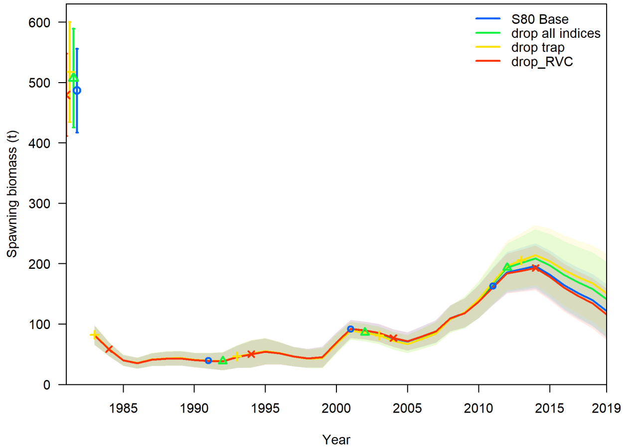
Figure 41. Results of a jackknife analysis for spawning biomass (metric tons) for the Puerto Rico Queen Triggerfish Base Model. There is some indication of bias as noted when the commercial trap index is removed from the model the estimate of SSB in the terminal year is higher. Shaded area represents the 95% confidence intervals about the model estimate.
